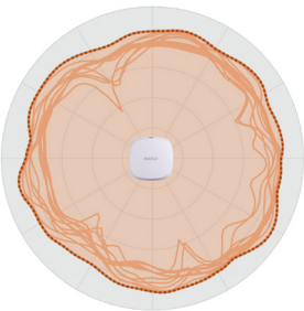
Selected BeamFlex Azimuth Patterns at 6 GHz
